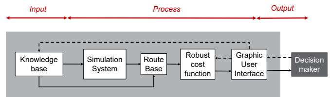
Agent-based Decision Support System's Structure
